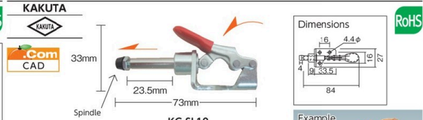
Toggle Clamp (lateral press type)
