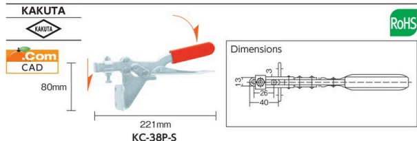
Toggle Clamp (downward press type/horizontal handle type)
