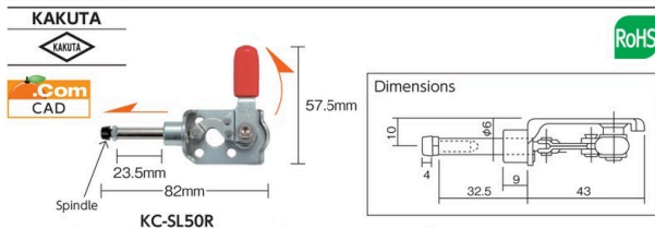
Toggle Clamp (lateral press type)
