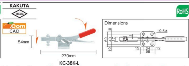
Toggle Clamp (downward press type/horizontal handle type)
