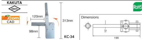
Toggle Clamp (downward press type/vertical handle type)
