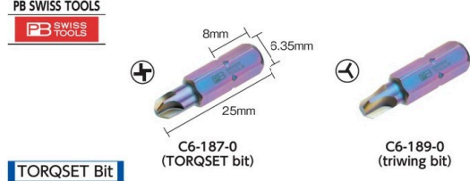
PB SWISS TOOLS C6-187-0 (TORQSET bit) C6-189-0 (trwing bit)
