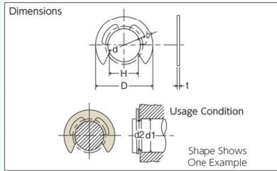
B92 Type (stainless steel)
