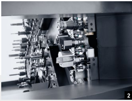
1: Tool chain magazine for up to 180 tools 2: Tool loading station with optimum accessibility from the front 3: Additional magazine for 6 oversized tools up to 700 mm length or ø200 mm (optional for all CTX gamma TC machines) 4: Disk magazine with 36 stations
