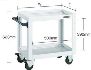
DLWS-662-W (white) (fixed type/flexible caster)
