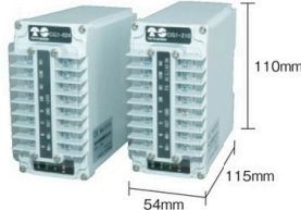
CG1-024 Controller (exclusive for DC) CG1-210 Controller (exclusive for AC)
