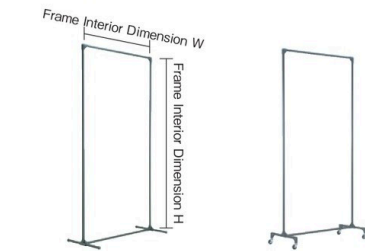
TF-1020K (stand alone type/fixed foot) TF-1020C (single unit, caster type)
